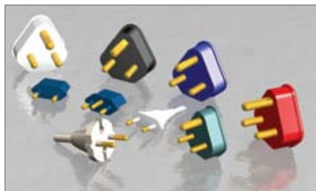
Fig. 2: SANS 164 - Family of plugs with 9 configurations
